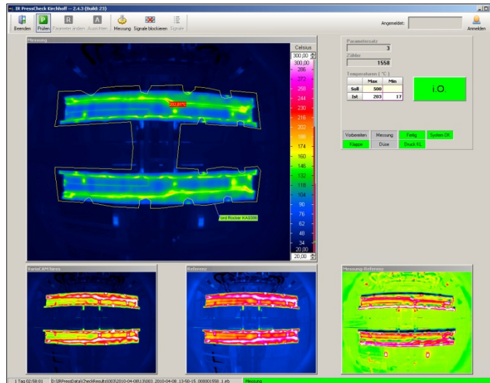
III. 2: Evaluation software IRBIS® 3 used for real-time display of thermograms from different sources (current measurement, live image, reference, difference) in automatic test mode
